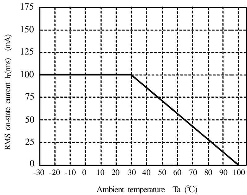
Fig.2 RMS on-state current vs. Ambient temperature
